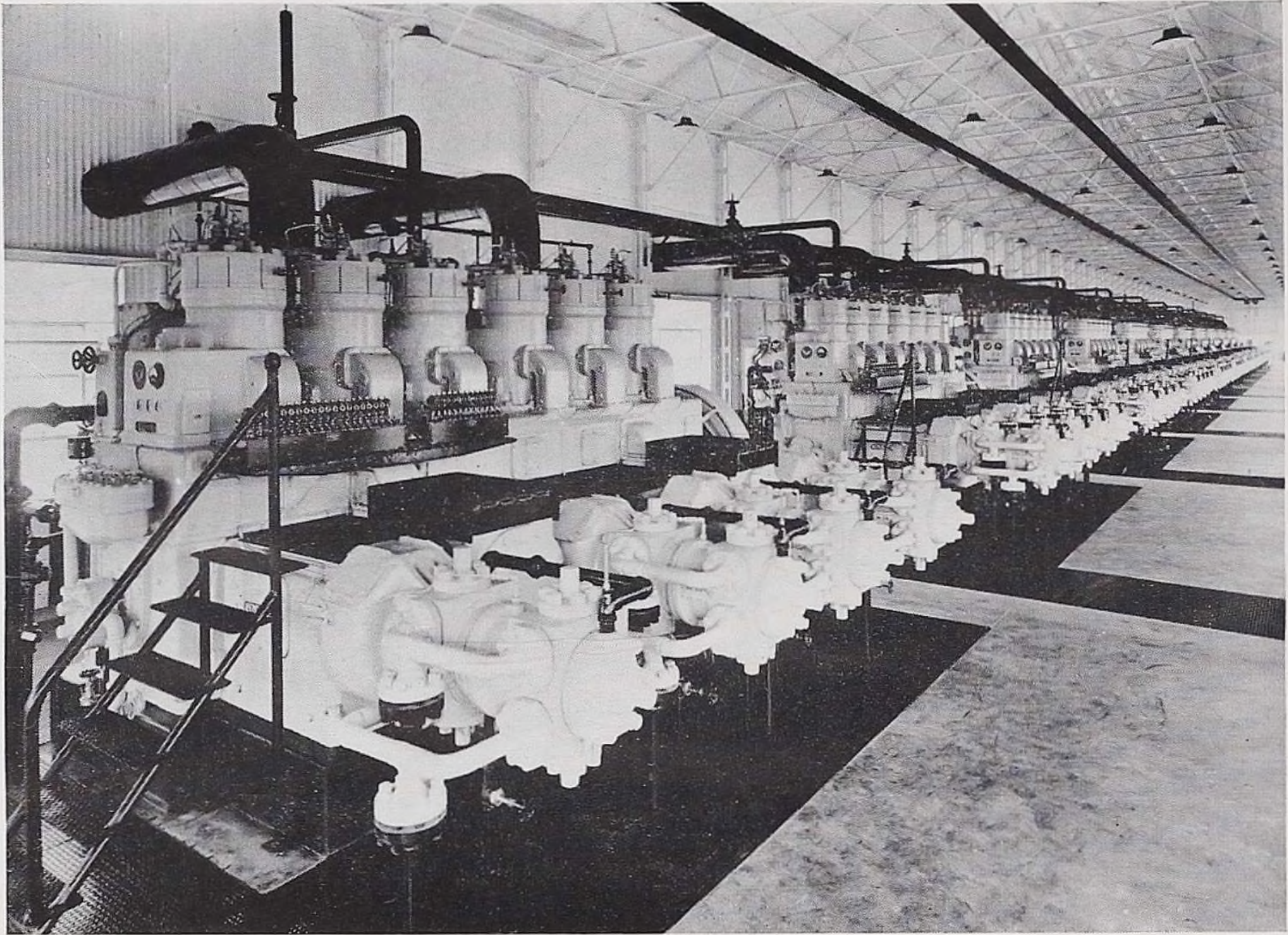
Clark 6-Cylinder "Angle" Compressors in Cotton Valley Gas Recycling Plant Located in Louisiana
